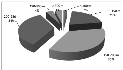
Fig. 1. Landslides distribution by elevation levels.
