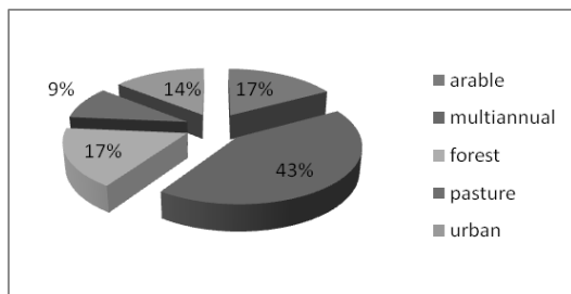
Fig. 5. Landslides distribution by land use types.
