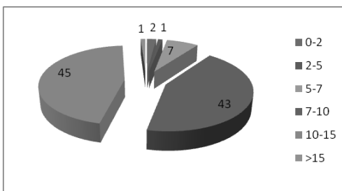
Fig. 2. Landslides distribution by slope angles.
